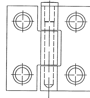
Narrow Butt Hinge With Loose Pin
