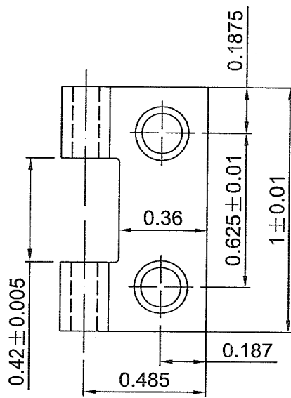
Narrow Butt Hinge With Loose Pin
